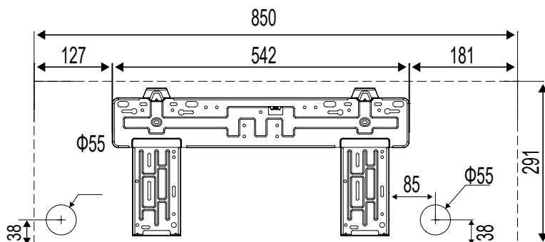
Multi-split : SMVH12B-3A2A3NG ( 12000 Btu )
