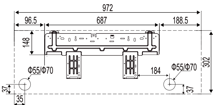
Mono-split : SMVH18B-4A2A3NG ( 18000 Btu )
