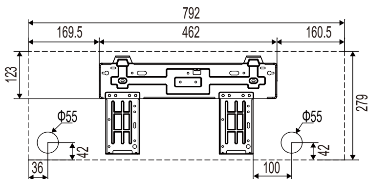
Multi-split : SMVH09B-2A2A3NG ( 9000 Btu )
