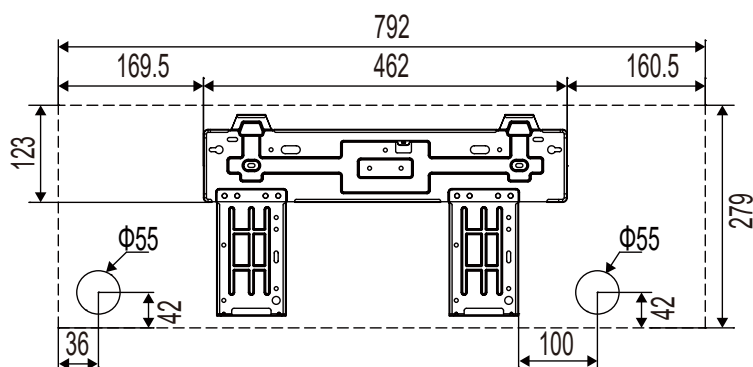
Mono-split : SMVH09B-2A2A3NH ( 9000 Btu ) SMVH12B-2A2A3NH ( 12000 Btu )
